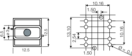
PCB layout (solder side)
