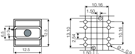
PCB layout (solder side)
